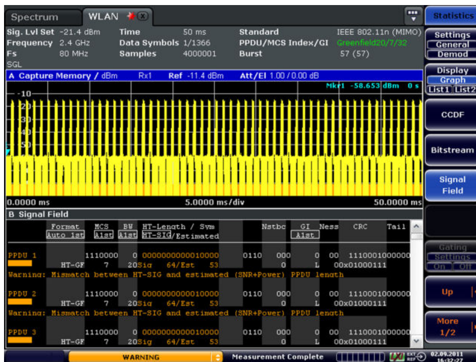
Fig. 3-7: The Signal Field measurement revealing a length conflict between the HT-SIG length and the length estimated from the PPDU power profile
